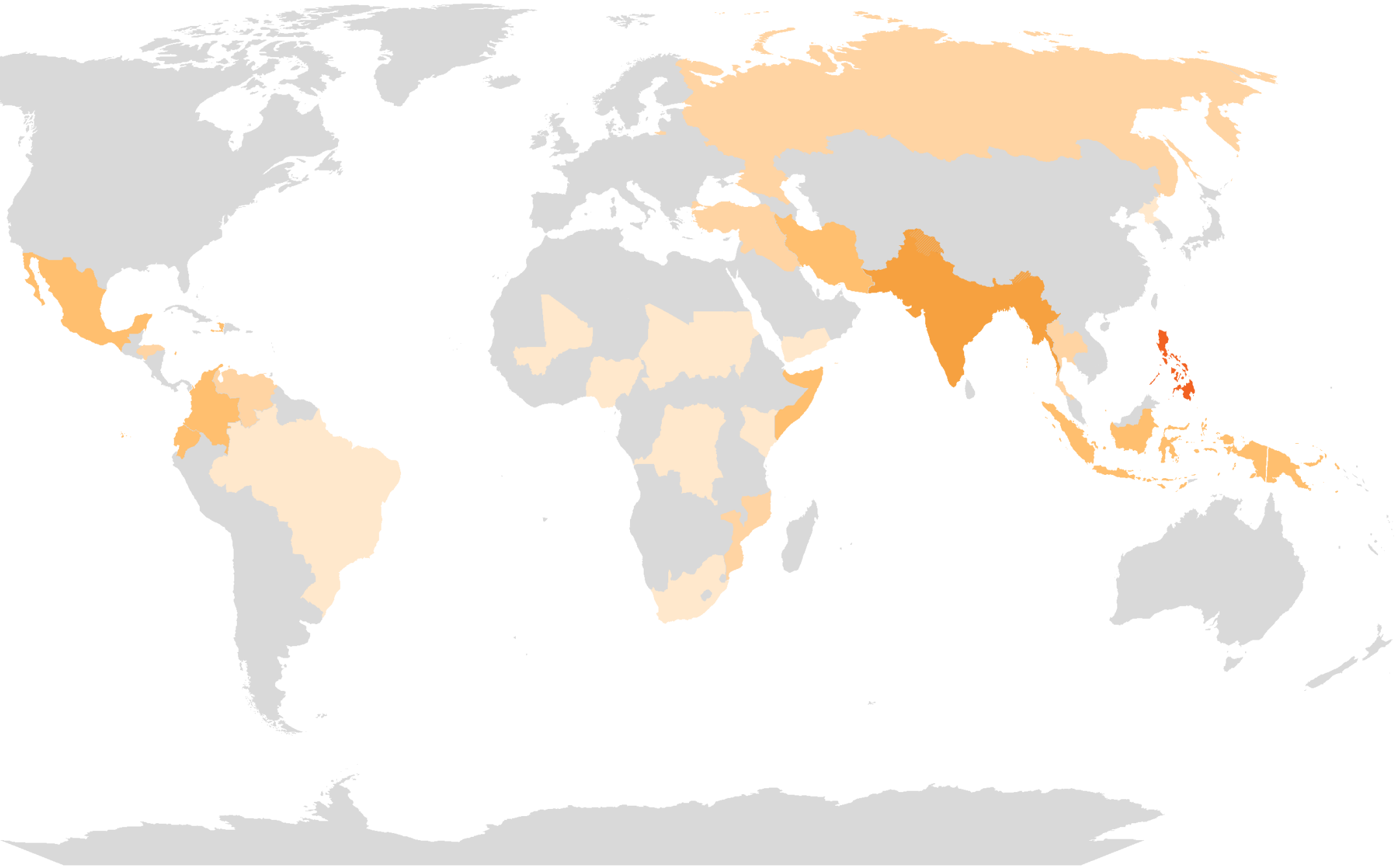
Figure 2. Countries with overlapping natural and human 'hazard and exposure' in the INFORM RISK Index 2025. Natural hazards cover earthquakes, river and coastal floods, tsunamis, tropical cyclones, droughts and epidemics (not all of which related to climate change). Human hazards are defined by projected conflict probability and current conflict intensity. Countries with both natural and human 'hazard and exposure' scores \geq 8 represented here as 5 (only the Philippines); \geq 7 here as 4; \geq 6 here as 3; \geq 5 here as 2; and \geq 4 here as 1. Countries with either natural or human 'hazard and exposure' scores below 4 are greyed on the map (adapted from European Commission, 2025).
